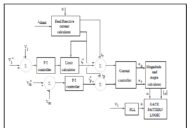
Fig.1.3: Block diagram of shunt VSC controller III. ACTIVE AND REACTIVE POWER CONTROL BY UPFC
