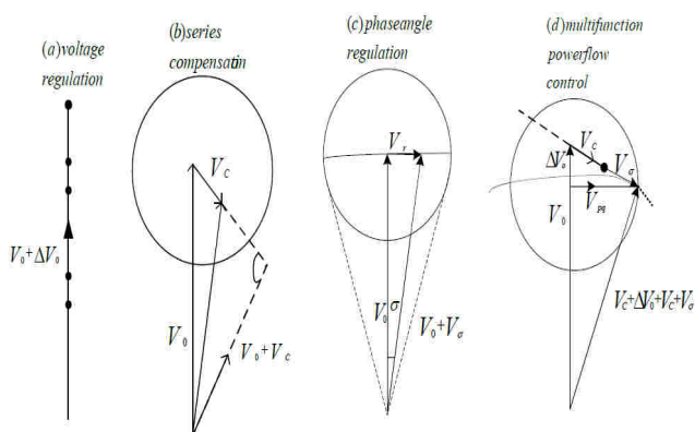
Fig.1.2 Basic UPFC control function. (a) Voltage Regulation (b) Series compensation (c) Angle regulation (d) Multi-function power flow controller
