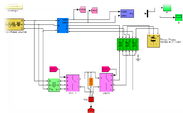
Fig.1.6:UPFC simulation modal
